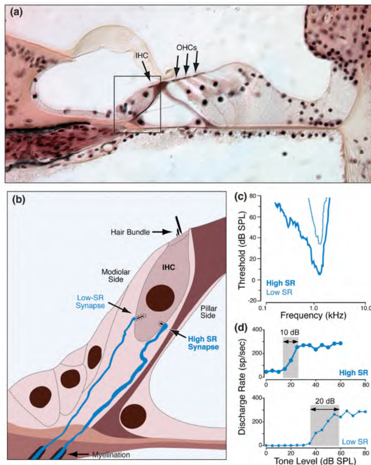
Figure 2. High- vs. low-SR auditory nerve fibers and their synaptic localization on the inner hair cell. (a) Light micrograph of the organ of Corti, as it appears in conventional histological material, stained with hematoxylin and eosin. Peripheral terminals of auditory nerve fibers (ANFs) in the inner hair cell (IHC) area (box) are not resolvable. (b) Schematic of type I peripheral terminals showing that fibers with high versus low spontaneous discharge rates (SRs) make synaptic contacts on opposite sides of the IHC. (c) High-SR fibers have lower thresholds than do low-SR fibers, as shown by these two tuning curves. (d) High-SR fibers have smaller dynamic ranges (grey box) than do low-SR fibers when stimulated with tone bursts at the characteristic frequency. dB SPL, decibels sound pressure level; OHC, outer hair cell.
