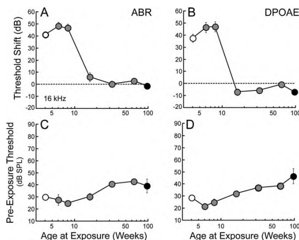
Figure 2. Vulnerability to noise decreases dramatically between 8 and 16 weeks of age. A, B , Maximum threshold shifts (i.e., shifts at 16 kHz) seen at 2 weeks after exposure by ABR ( A ) and DPOAE ( B ) for all ages at exposure. C, D , In unexposed control ears, thresholds at 16 kHz do not show large change between 8 and 16 weeks. Data are means \pm SE and are plotted as a function of age on a logarithmic scale. For the numbers of animals in each group, see Table 1.
